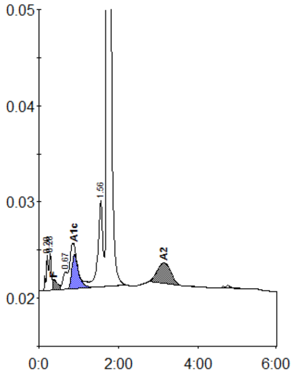
Peak table - ID: 05180007
