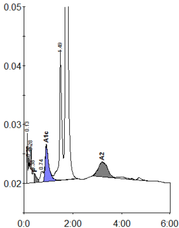
Peak table - ID: 13060002
