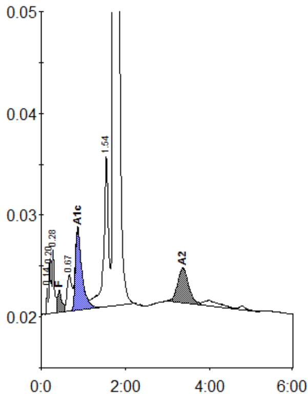
Peak table - ID: 06210021
