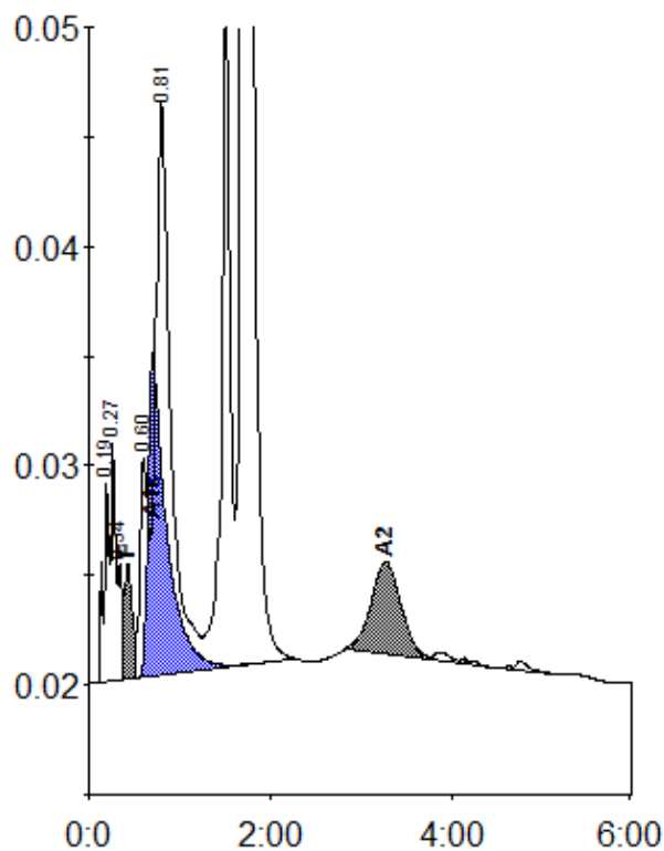
Peak table - ID: 0631
