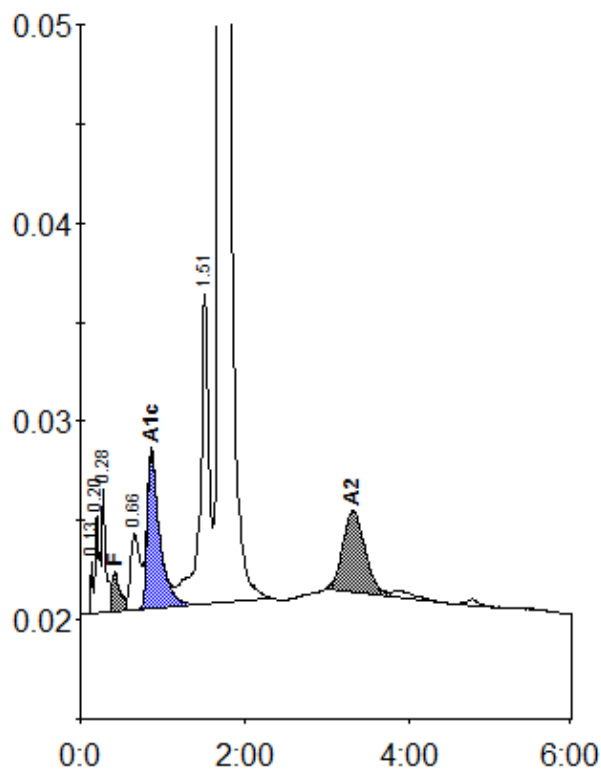
Peak table - ID: 10160085
