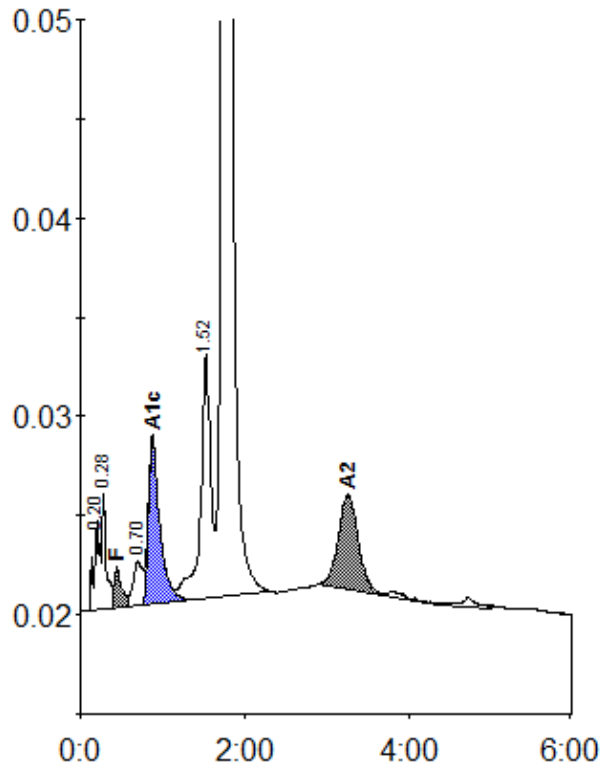
Peak table - ID: 06290016
