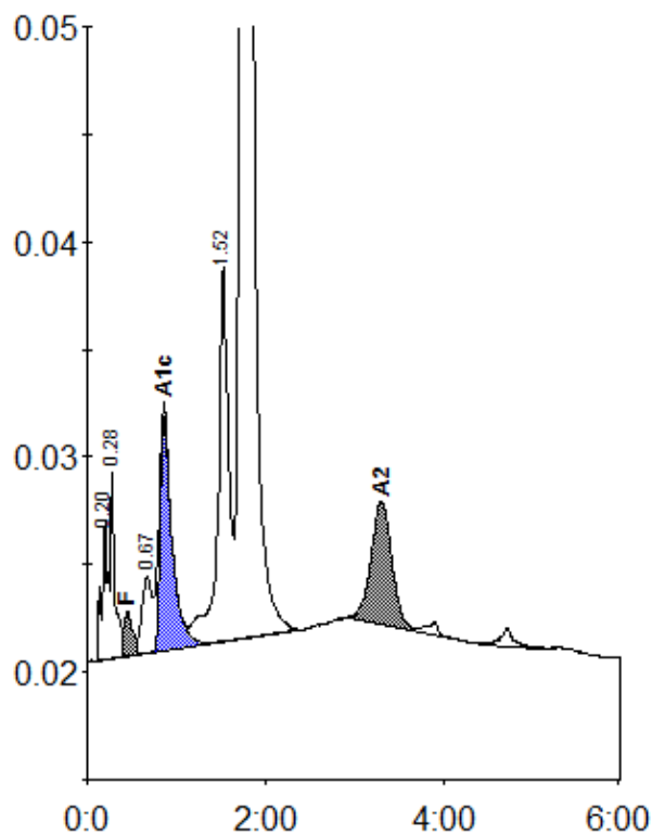
Peak table - ID: 11010003
