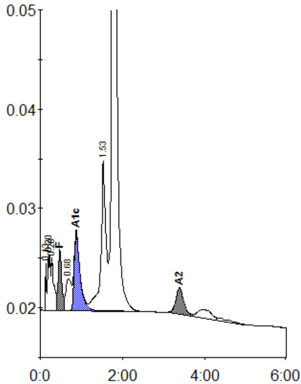
Peak table - ID: 25120026
