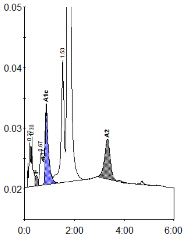
Peak table - ID: L3901337
