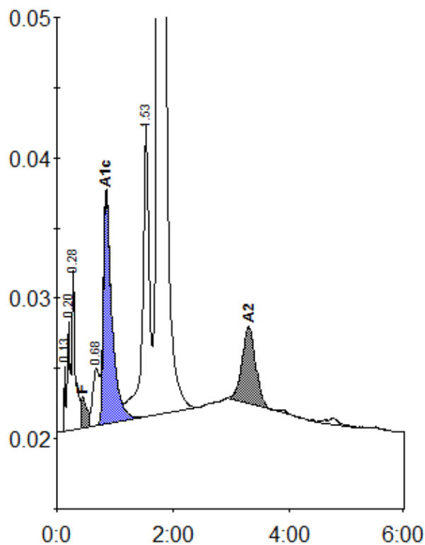
Peak table - ID: 11300021
