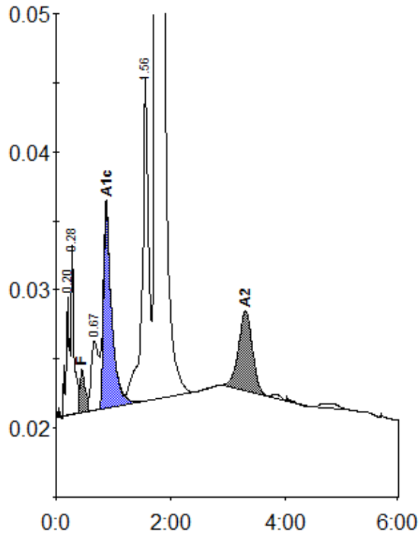
Peak table - ID: A0115310
