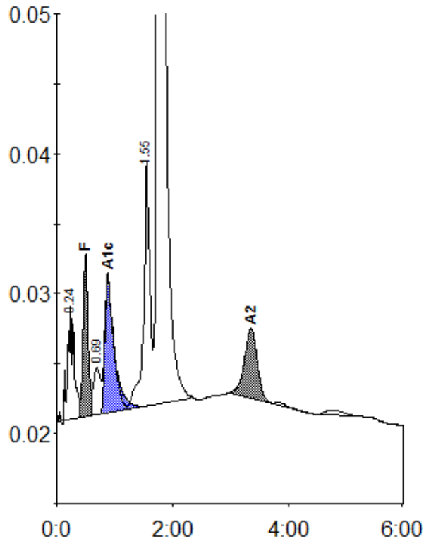
Peak table - ID: 21260006
