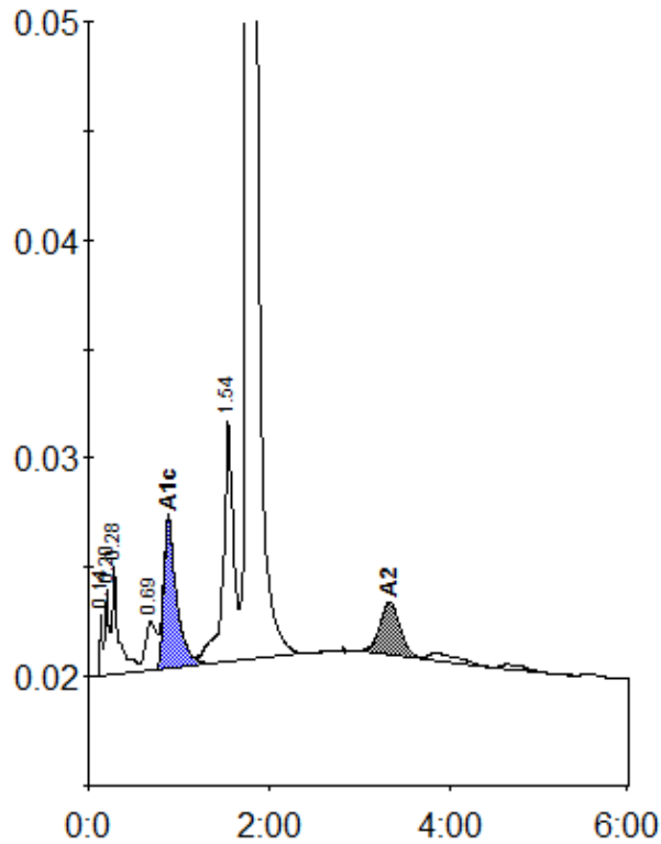
Peak table - ID: Z0155039
