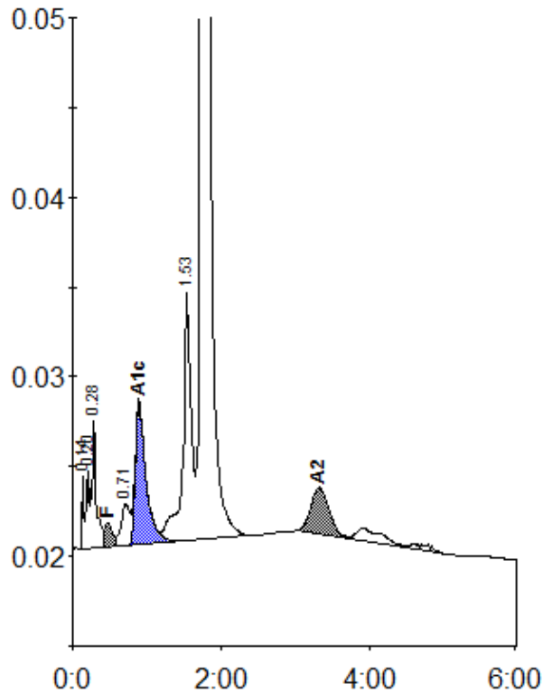
Peak table - ID: 22290003
