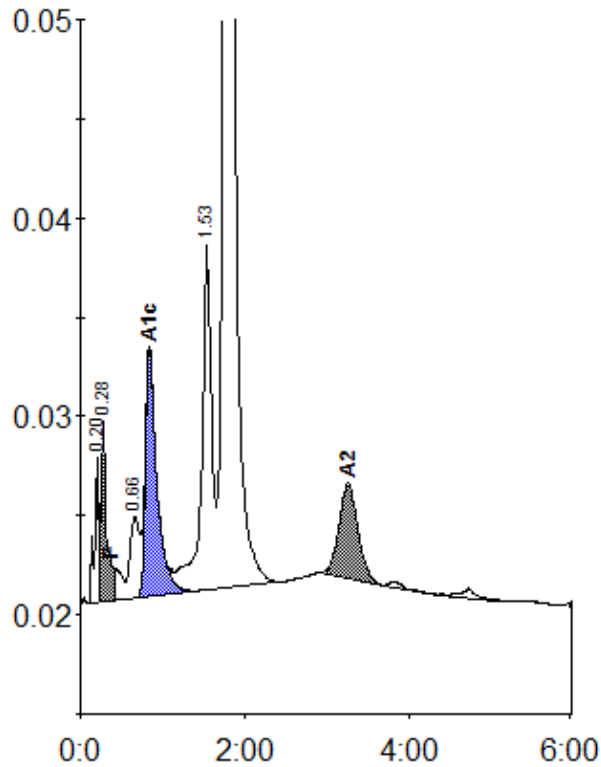
Peak table - ID: Z0115830
