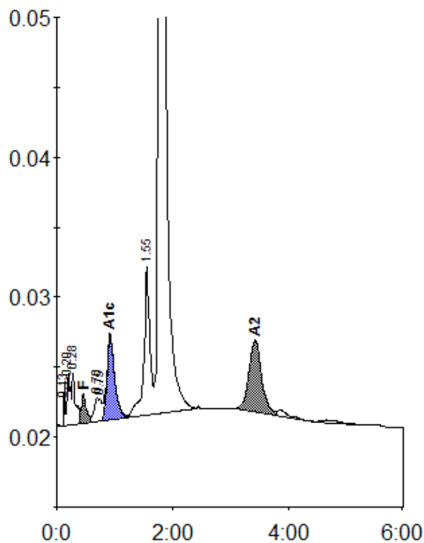
Peak table - ID: 10120077
