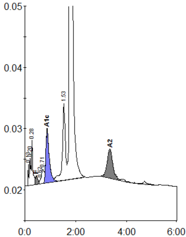
Peak table - ID: 20310007
