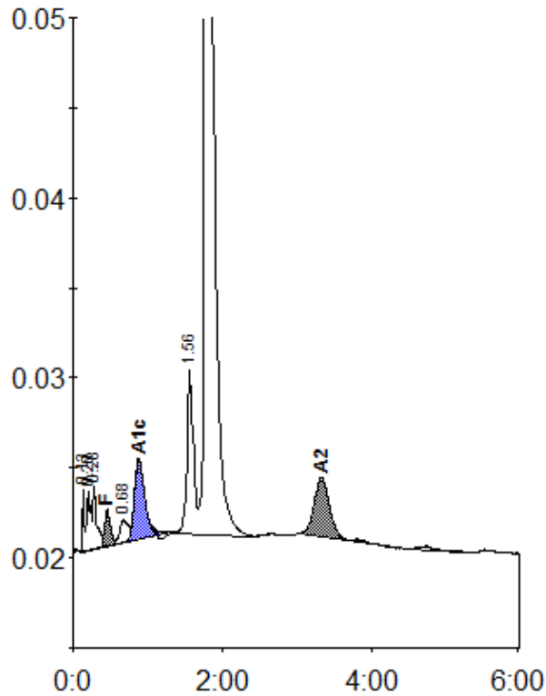
Peak table - ID: A0586431
