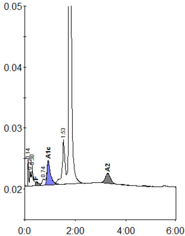
Peak table - ID: 24500520
