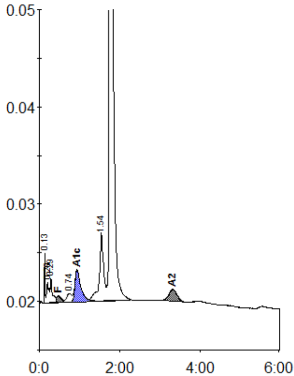
Peak table - ID: Y0410527
