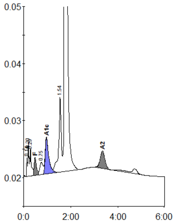
Peak table - ID: Y0424791
