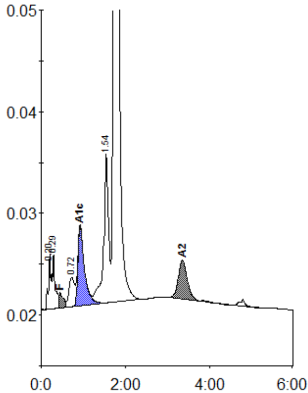
Peak table - ID: WCD15487
